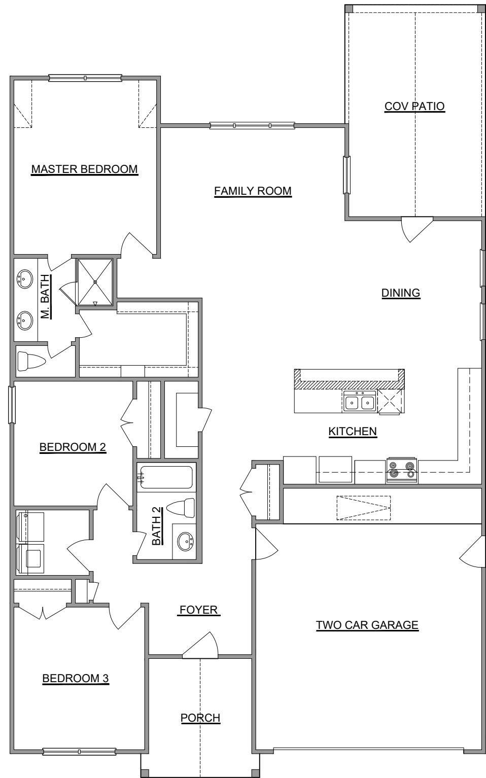
FLOOR PLAN
